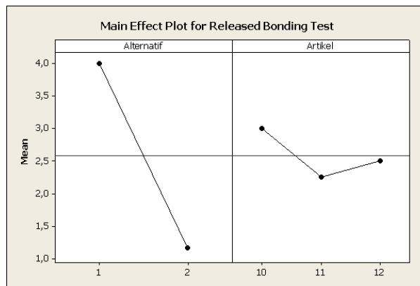
Fig 13. Main Effect Plot for Released Bonding Test
