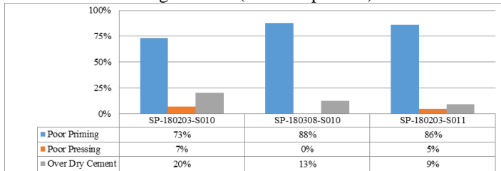
Fig 7. Data of the Rejected Bonding Accelerator LS Shoe June - August 2018 (Customer Return)
