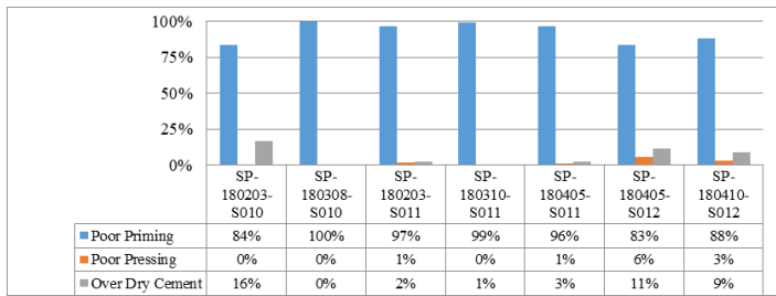
Fig 6. Data of the Rejected Bonding Accelerator LS Shoe June - August 2018 (Final Inspection)
